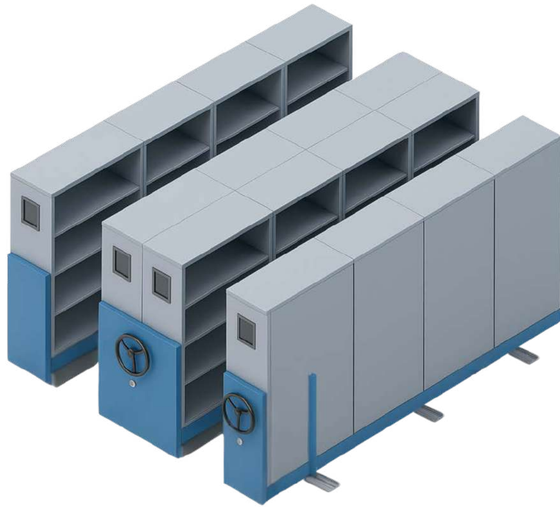
CDSH_MCS_007 W x D 900 x 450 / 900 x 600 / 1000 x 450 H = 2100 / 1800 ±10
